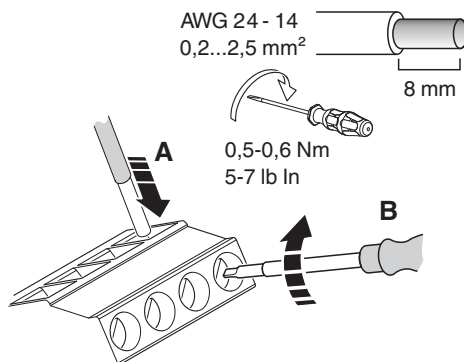
Figure 3 Screw connection
