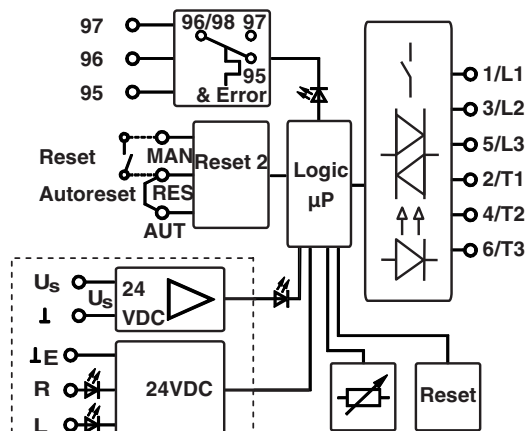
Figure 4 Block diagram
