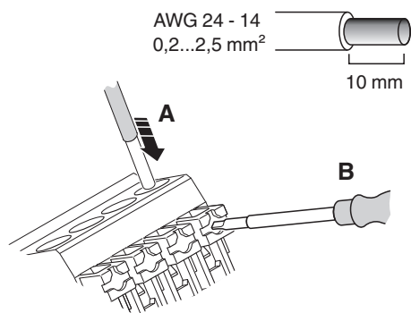
Figure 2 Push-in connection
