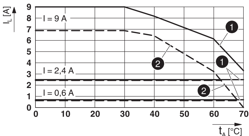
Figure 7 Derating curve
