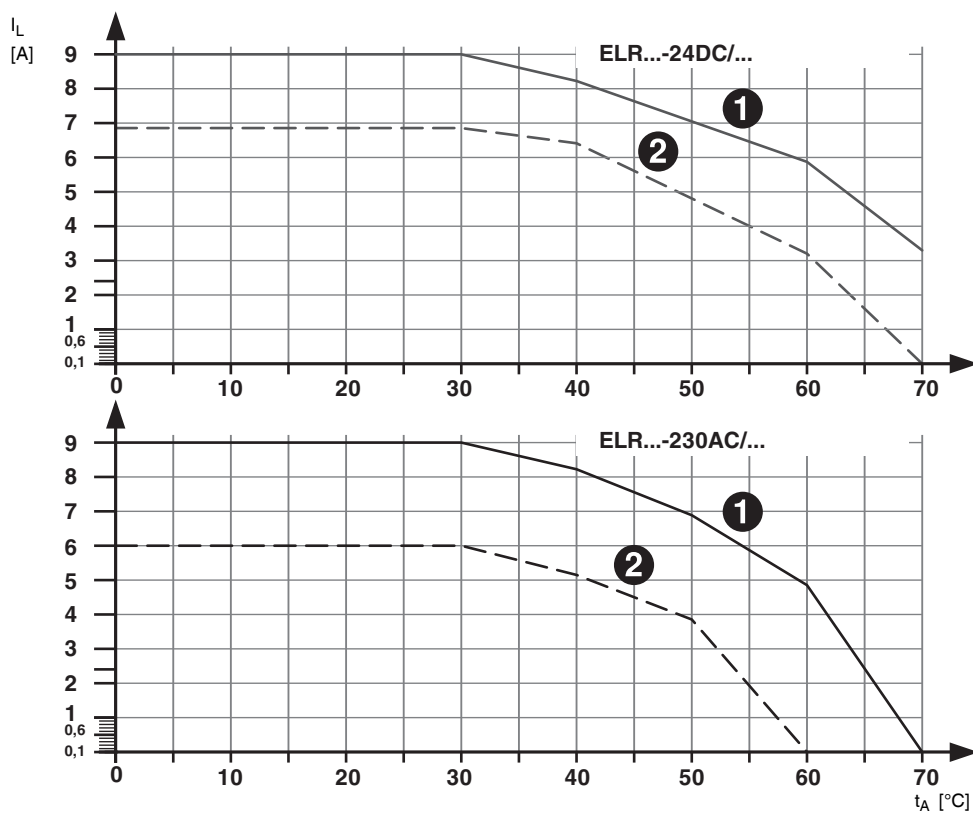
Figure 1 Derating curves for 100% operating time
