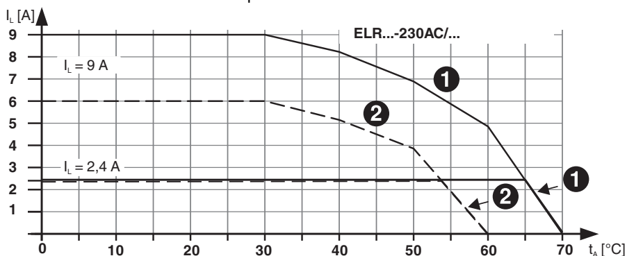
Figure 6 Derating curve
