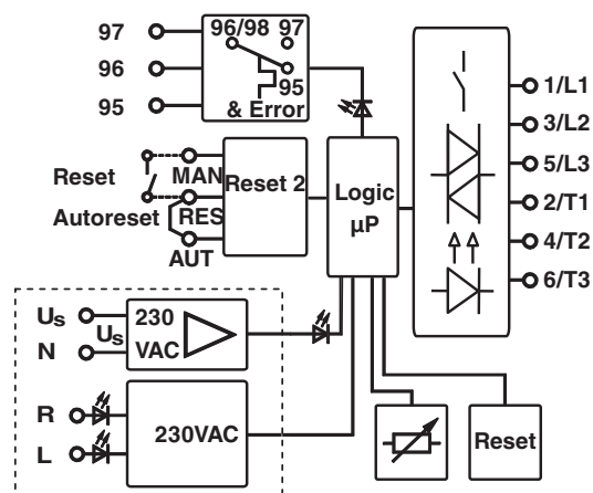
Figure 3 Block diagram
