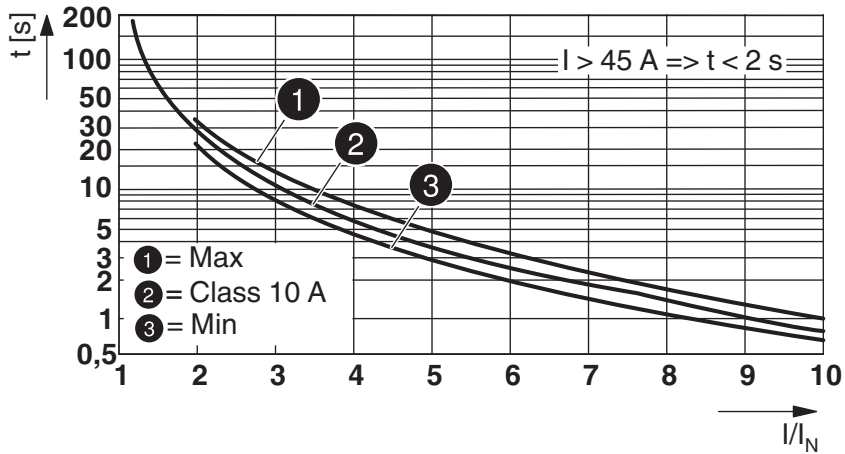
Figure 4 Trigger characteristic
