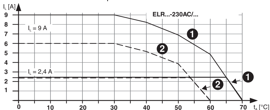
Figure 5 Derating curve
