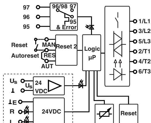
Figure 4 Block diagram
