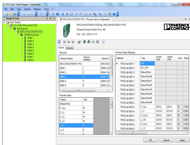
Figure 20 Device selection
