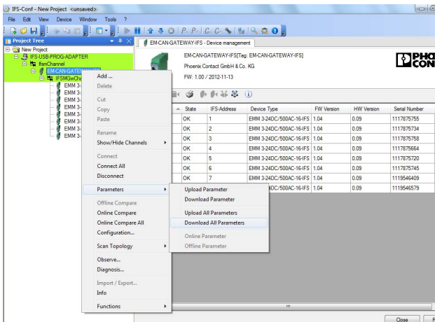
Figure 16 Downloading parameters
