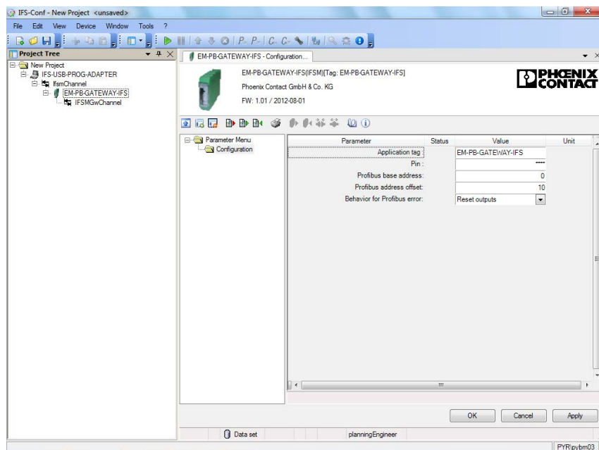
Figure 33 Settings EM-PB-GATEWAY-IFS
