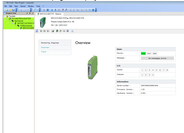
Figure 24 Status overview
