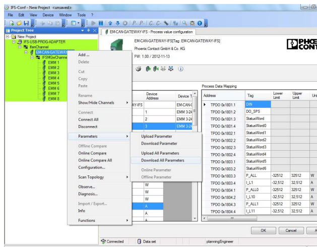
Figure 21 Writing project data to the modules
