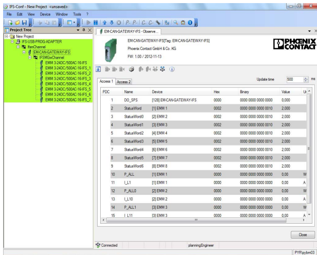
Figure 23 Displaying process values in the monitoring window
