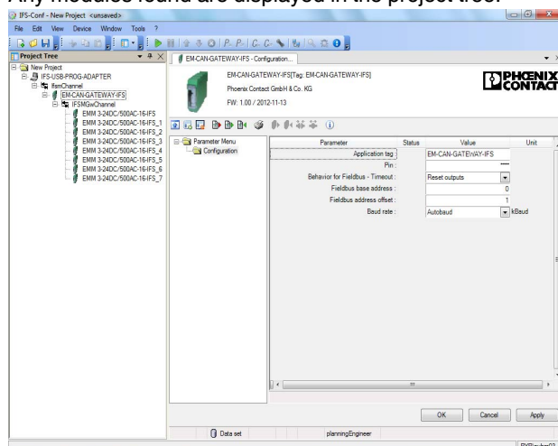
Figure 12 Project tree
