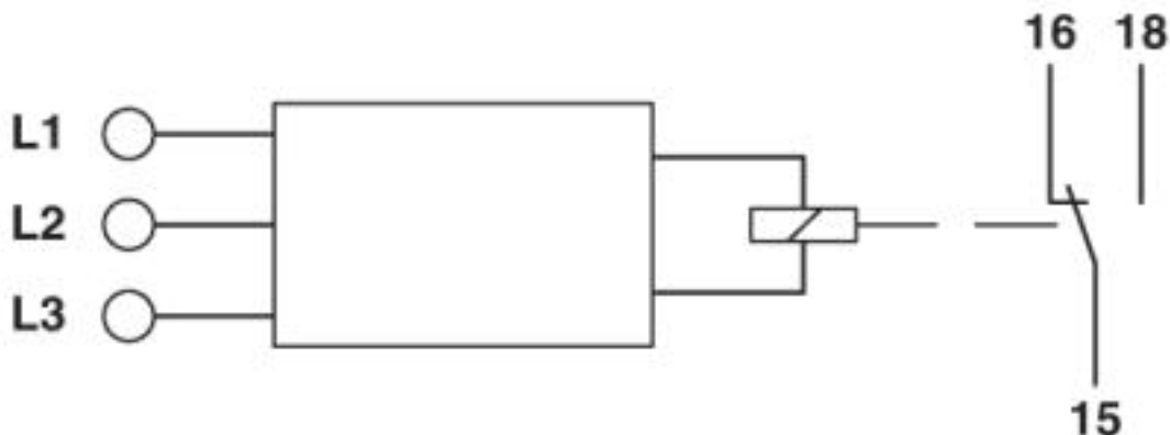
Block diagram
