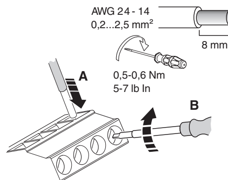
Figure 3 Screw connection
