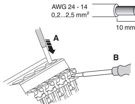
Figure 2 Push-in connection
