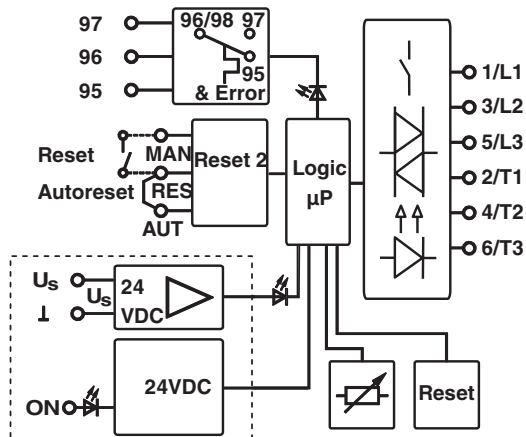
Figure 4 Block diagram
