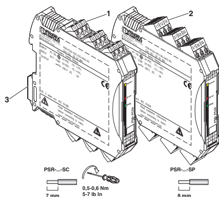
Figure 5 Connection versions
