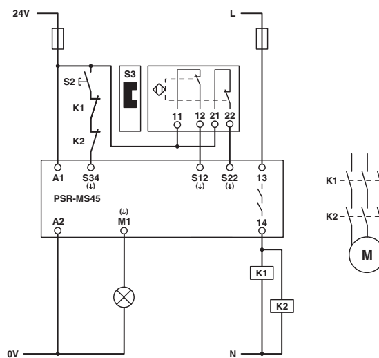
Figure 18 Magnetic switch monitoring/manual, monitored start
