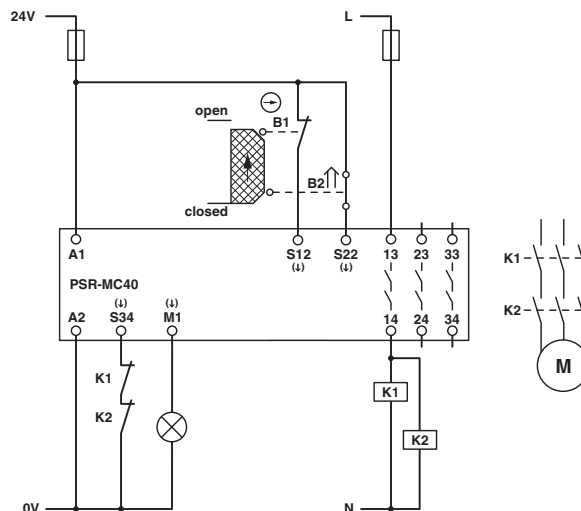
Figure 51 Safety door monitoring/automatic start
