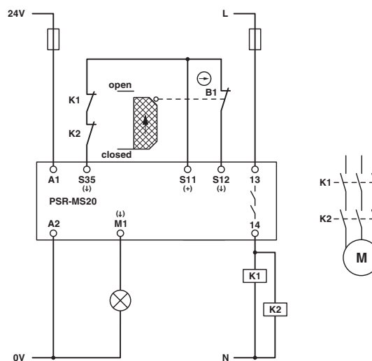
Figure 2 Safety door monitoring/automatic start
