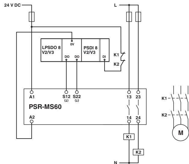
Figure 22 Two-channel control via LPSDO module
