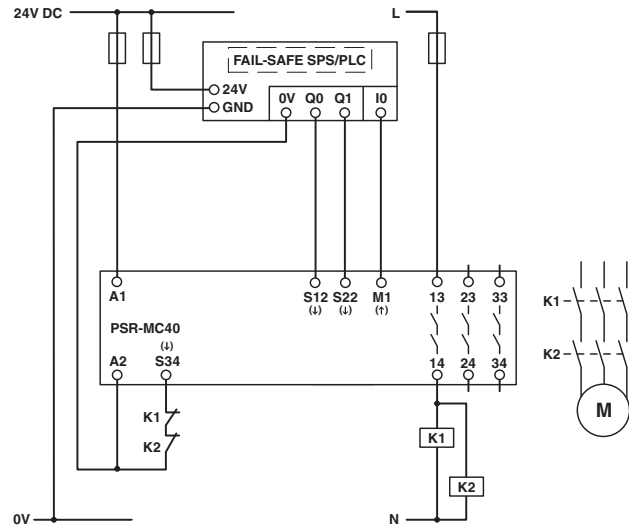
Figure 55 Connection to failsafe PLC/automatic start
