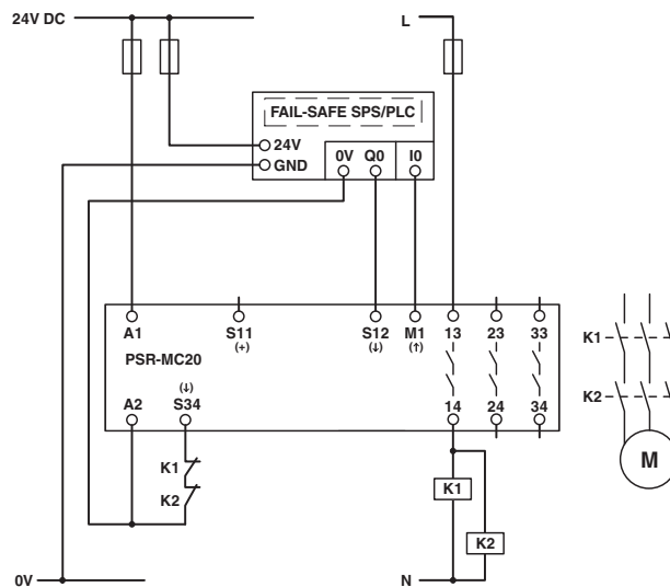
Figure 28 Connection to failsafe PLC/automatic start
