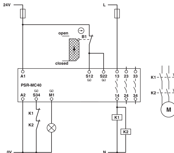
Figure 53 Single-channel safety door monitoring/automatic start
