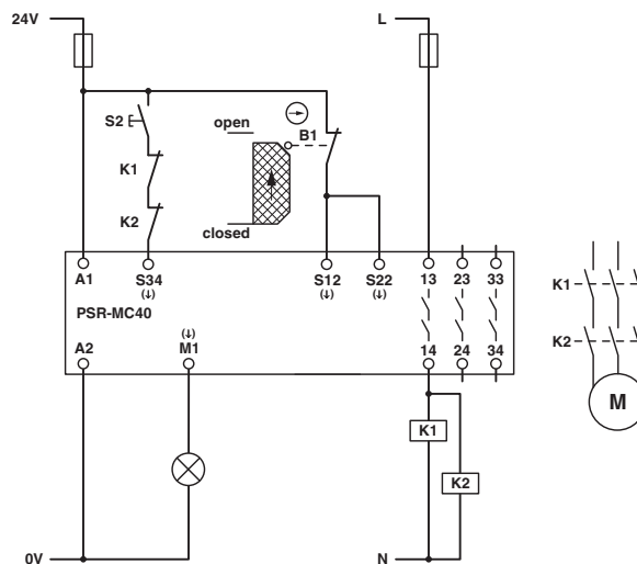
Figure 54 Single-channel safety door monitoring/manual, monitored start
