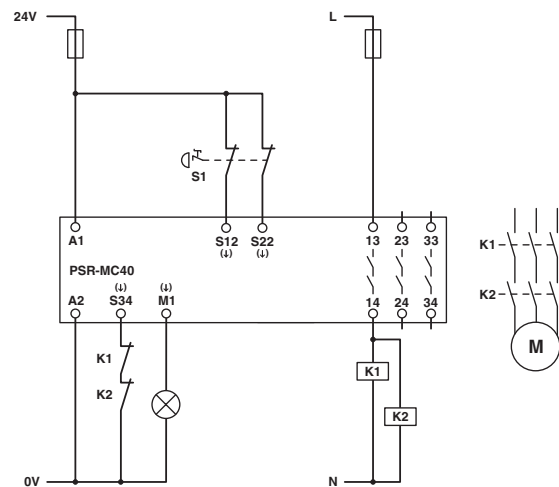
Figure 49 Emergency stop monitoring/automatic start
