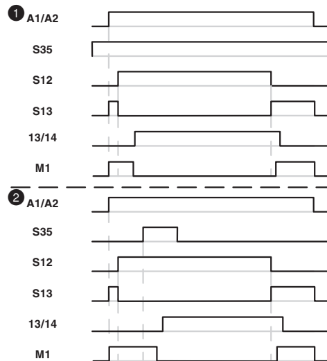
Figure 1 Time diagram PSR-MS50
