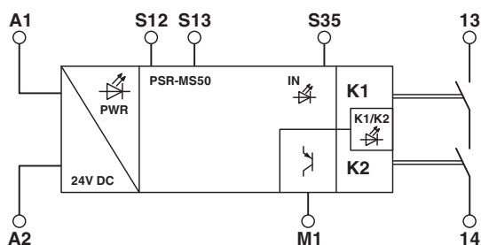
Figure 3 Block diagram PSR-MS50
