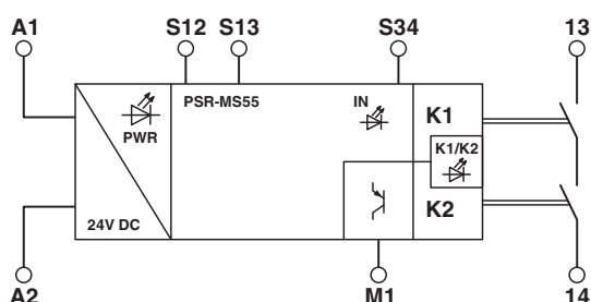
Figure 4 Block diagram PSR-MS55
