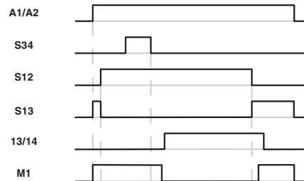
Figure 2 Time diagram PSR-MS55
