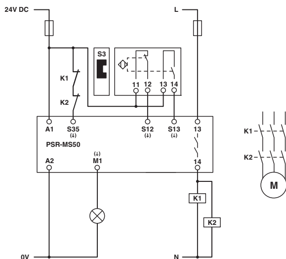
Figure 12 Magnetic switch monitoring/automatic start
