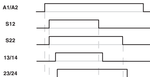
Figure 1 Time diagram
