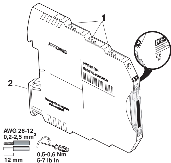
Figure 5 Connection versions
