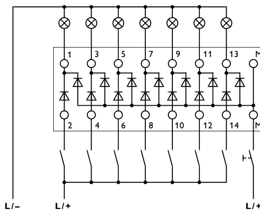
Figure 1 Lamp test circuit (EMG 45-DIO14M/LP)
