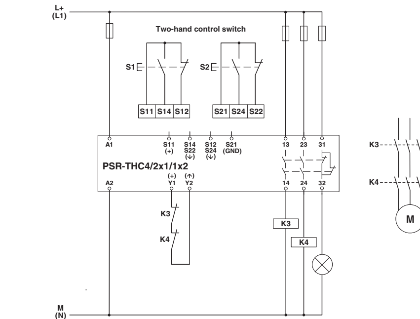
Figure 5-25 Two-hand control device monitoring PSR-THC4/2x1/1x2
