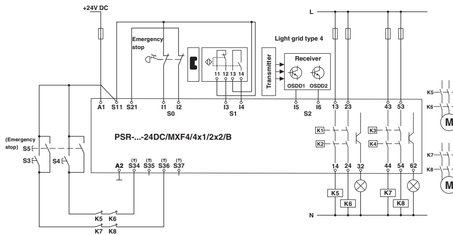
Figure 6-5 Two-channel emergency stop, safety door, and light grid monitoring PSP-MXF4/4X1/2X2/B
