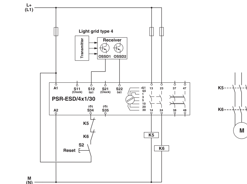
Figure 5-10 Two-channel light grid monitoring with manual reset PSR-ESD/4x1/30
