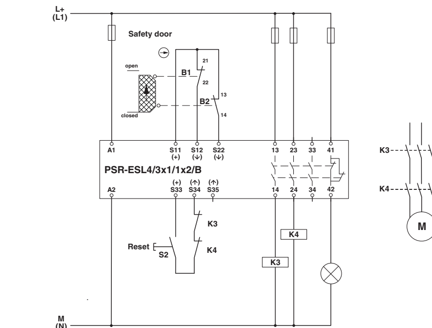
Figure 5-20 Two-channel safety door monitoring with manual reset PSR-ESL4/3x1/1x2/B
