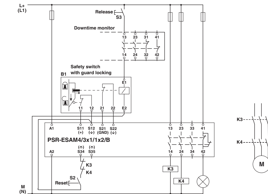
Figure 5-16 Two-channel safety door monitoring with manual reset PSR-ESAM4/3x1/1x2/B
