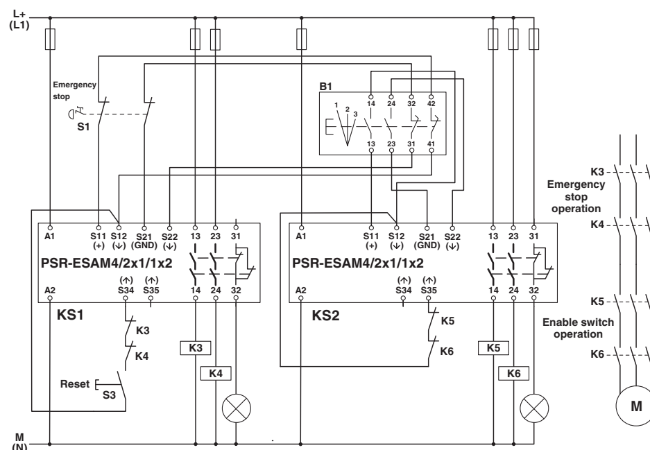
Figure 5-23 Three-stage enable switch with two-channel emergency stop monitoring PSR-ESAM4/2x1
