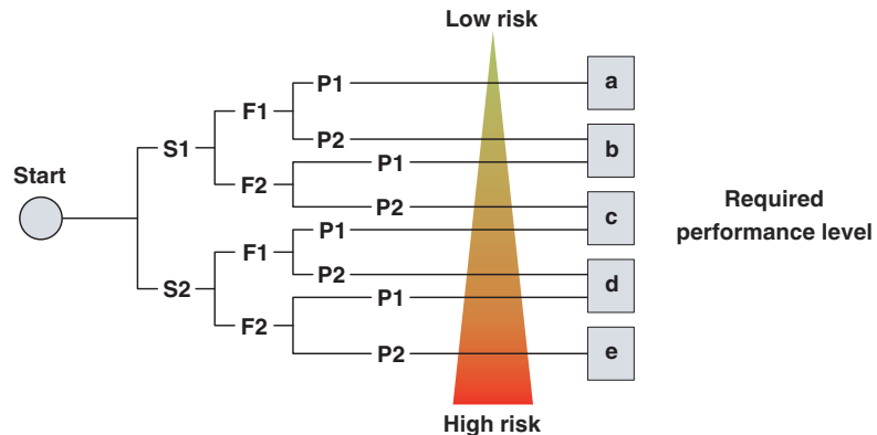
Figure 2-2 Risk graph (in accordance with EN 13849-1)
