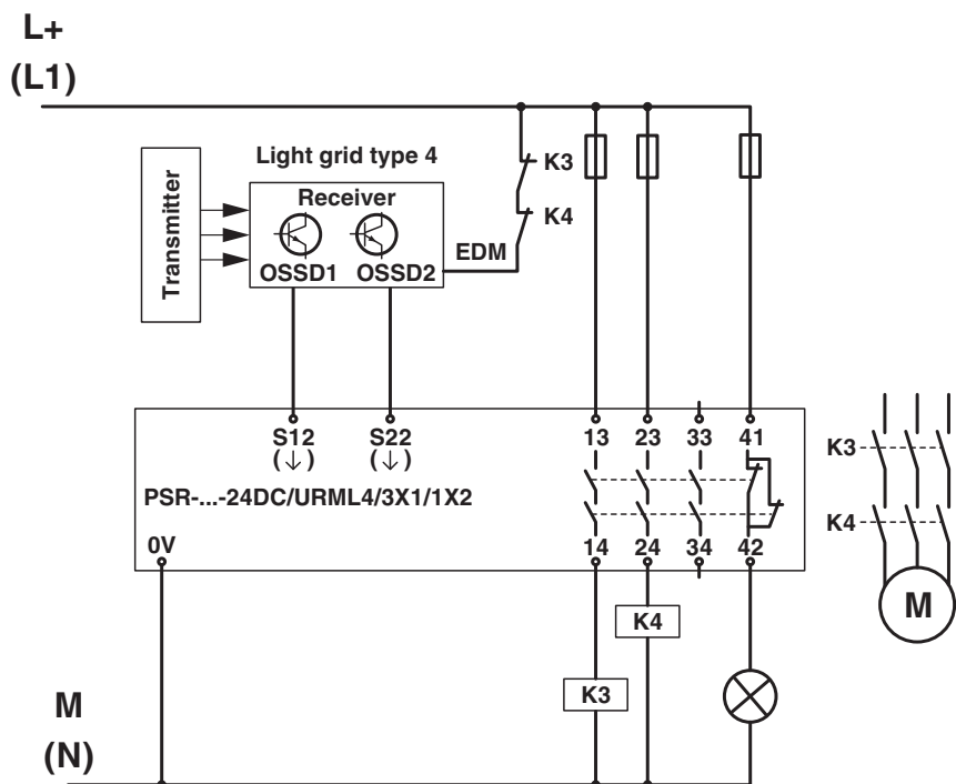
Figure 5-28 Application example: light grid monitoring PSR-URML4/3x1/1x2/B
