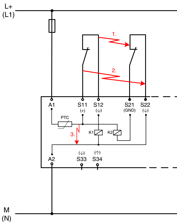
Figure 3-1 Cross-circuit detection
