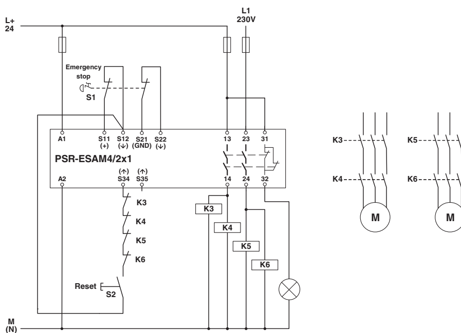
Figure 5-4 Two-channel emergency stop monitoring with manual reset PSR-ESAM4/2x1/1x2
