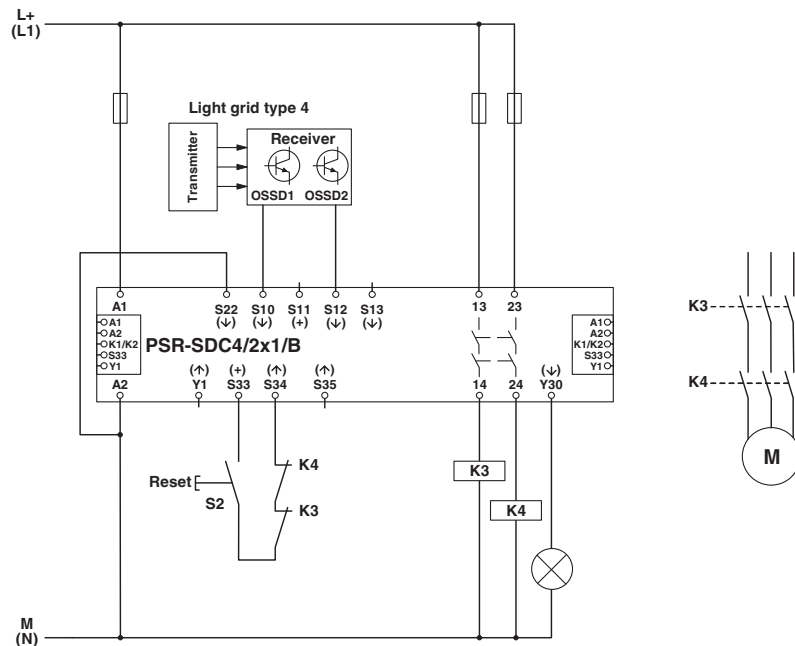
Figure 7-3 Two-channel light grid monitoring with manual reset PSR-SDC4/2x1/B
