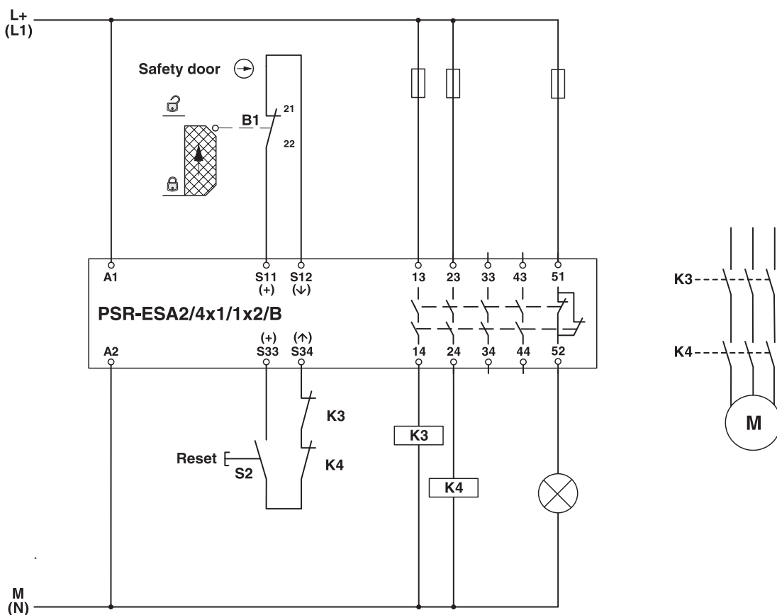
Figure 12 Single-channel safety door monitoring/manual start
