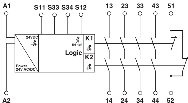
Figure 3 Block diagram
