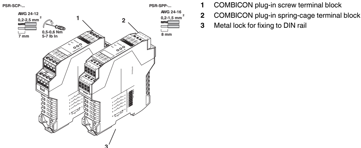
Figure 6 Connection versions
