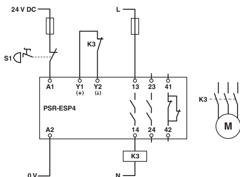
Figure 12 Single-channel emergency stop monitoring/ autostart
