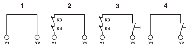
Figure 9 Start and feedback circuit connection variants
