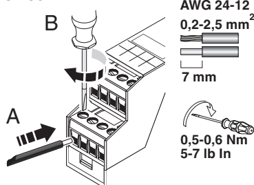
Figure 6 Connecting the cables for PSR-SCP-... (Screw terminal block)
