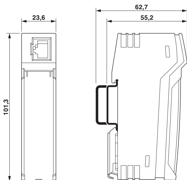
Figure 1 Dimensions
