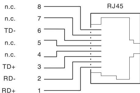
Figure 9 Pin assignment
