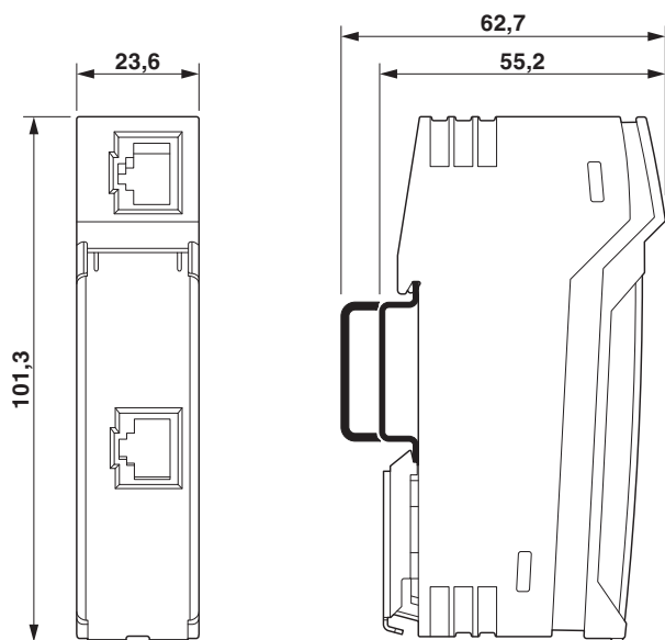
Figure 2 Dimensions
