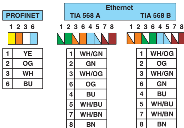
Figure 10 Terminal assignment
