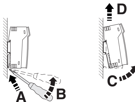
Figure 8 Removal
