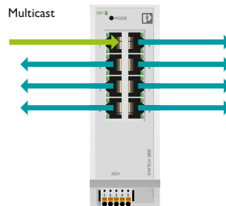
Without IGMP snooping
