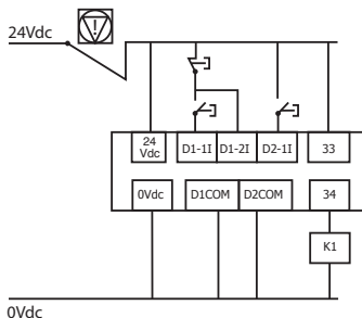
3 wire Control Diagram 24Vdc control supply ( U_c ) and digital input ( U_i ) programming.
