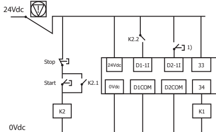
24Vdc ( U_c ) and ( U_i ) user programmable control diagram.
