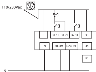
3 Wire Control Diagram 110/230Vac control supply ( U_c ) and digital input ( U_i ) programming.
