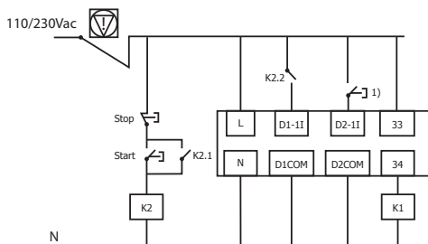
110/230Vac ( U_c ) and ( U_i ) user programmable control diagram
