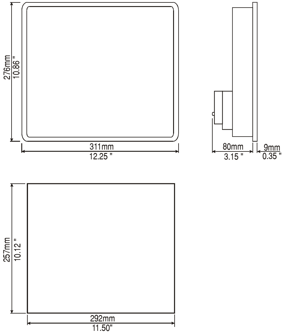
Figure 18 - Dimensions
