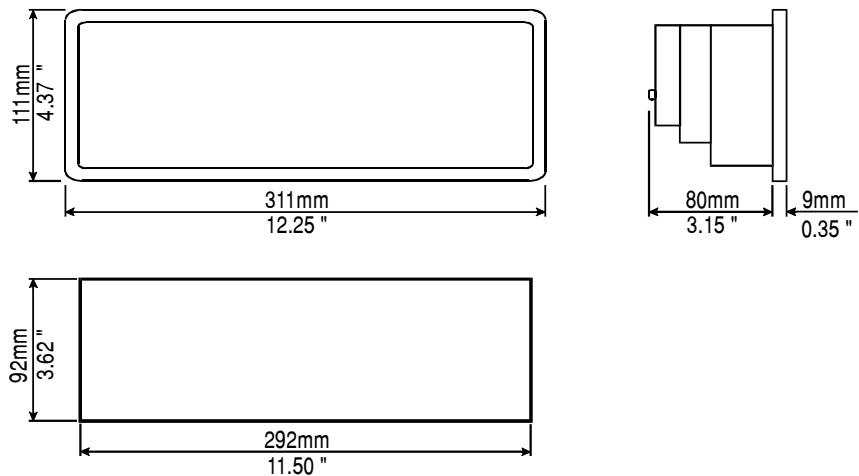
Figure 8 - Dimensions
