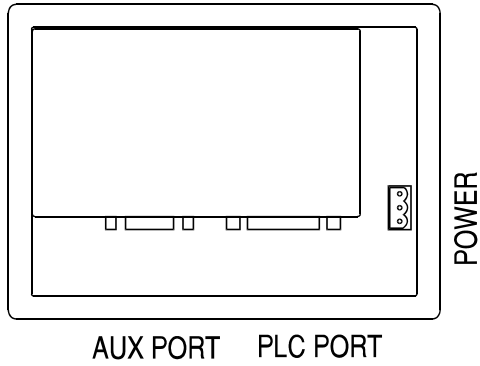
Figure 20 - Connectors
