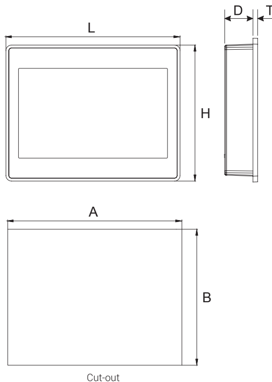
Cut-out
