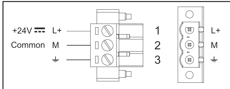
Fig. 6.1 - Power supply terminal block
