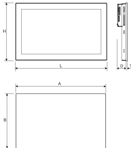
Cut-out
