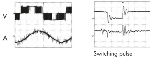
Switching pulse
