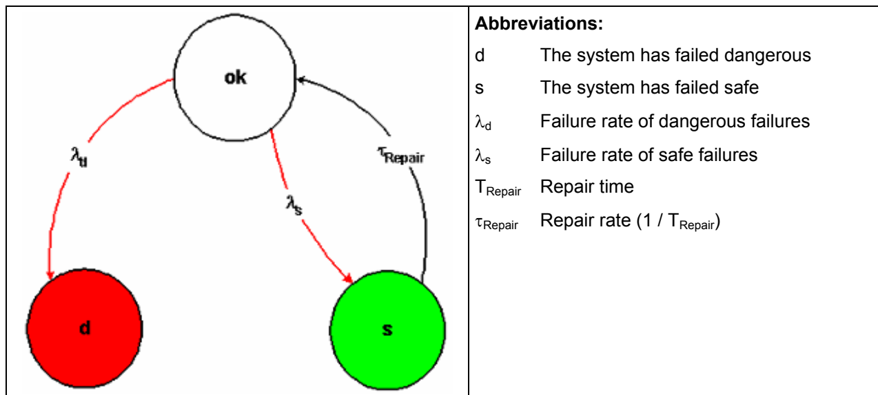
Figure 4: Markov model
