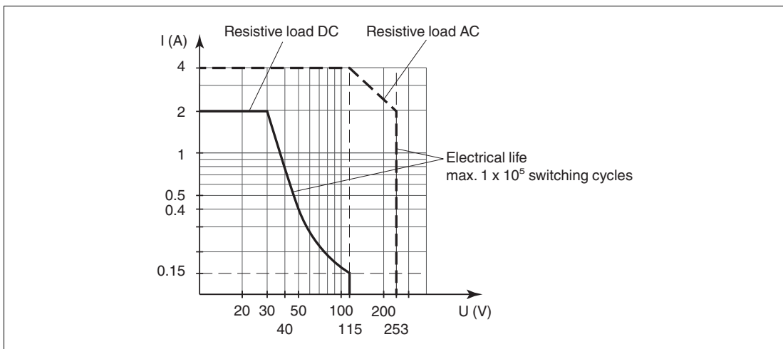
Figure 3.2 Maximum switching power of KCD2-SR-(Ex)*(.LB)(.SP)
