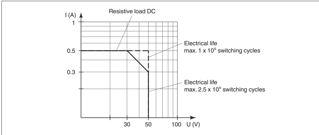
Figure 3.1 Maximum switching power of HiC282*
