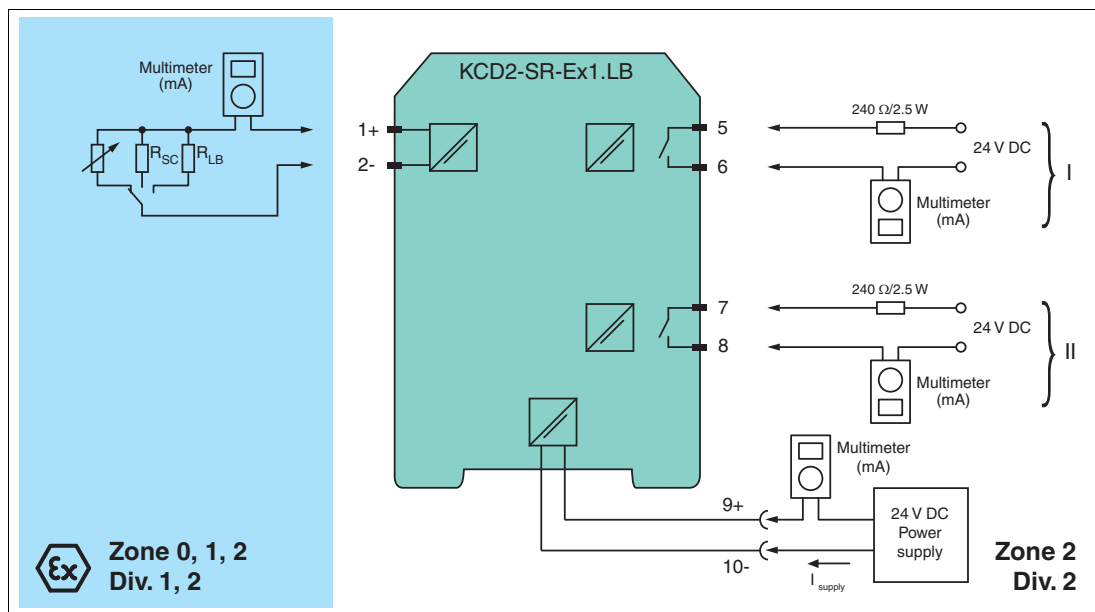
Figure 5.1 Proof test set-up for KCD2-SR-(Ex)1.LB(.SP)
