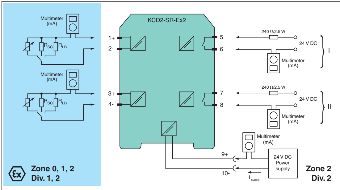
Figure 5.2 Proof test set-up for KCD2-SR-(Ex)2(.SP)
