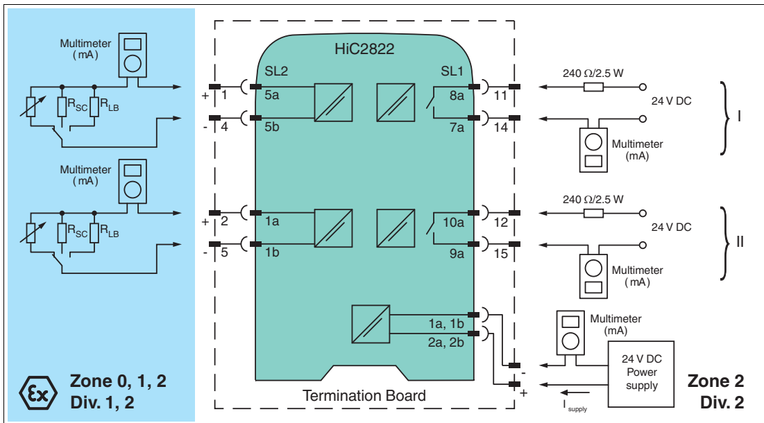
Figure 5.3 Proof test set-up for HiC2821, HiC2822
