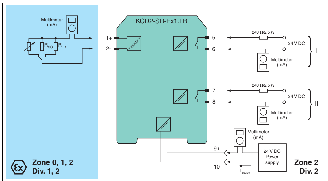
Figure 5.1 Proof test set-up for KCD2-SR-(Ex)1.LB(.SP)
