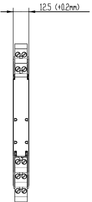
Version with high screw terminals
