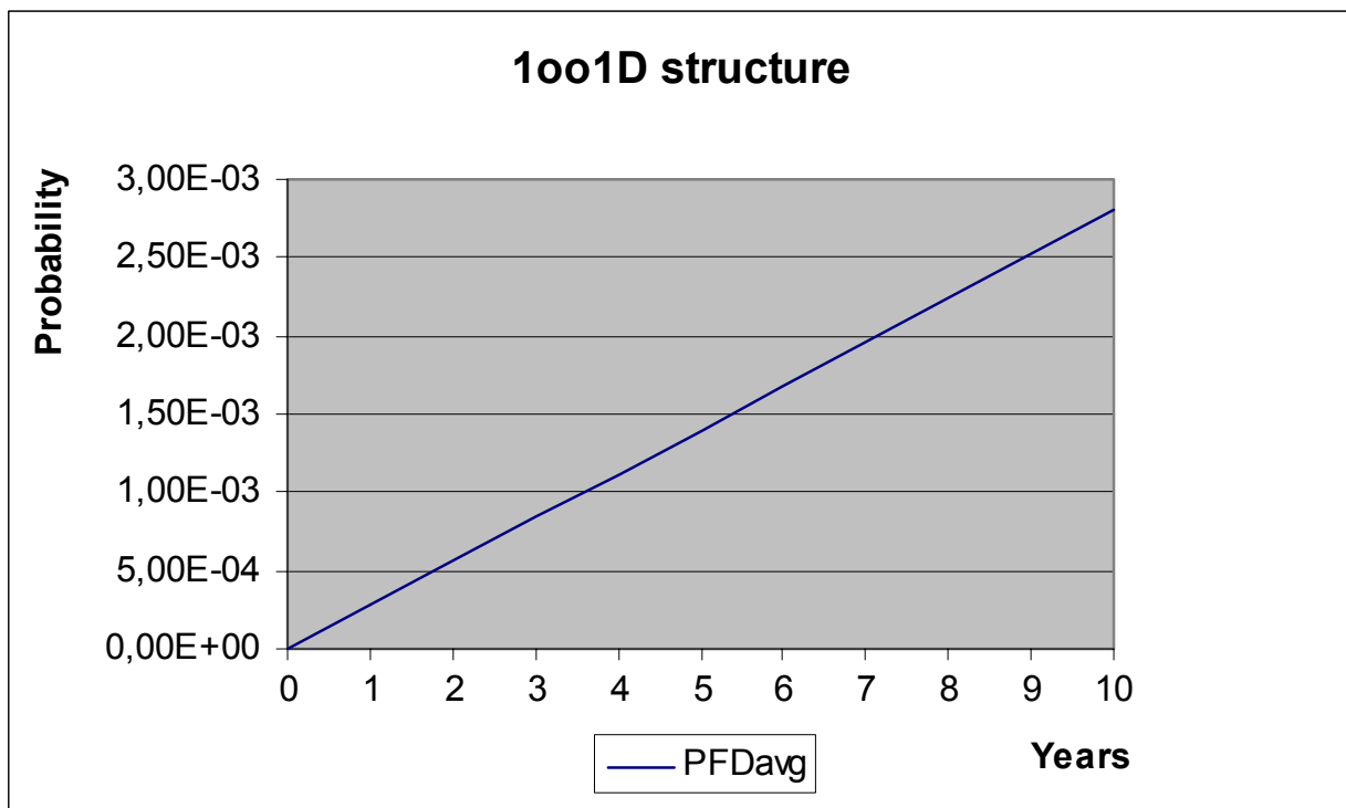
Figure 7: PFD_{AVG}(t)
