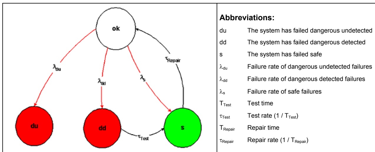
Figure 4: Markov model for a 1oo1D structure
