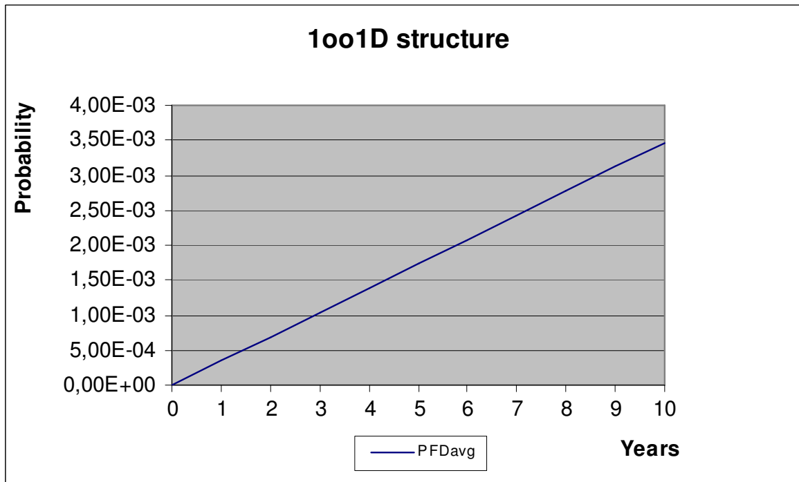
Figure 8: PFD_{AVG}(t)
