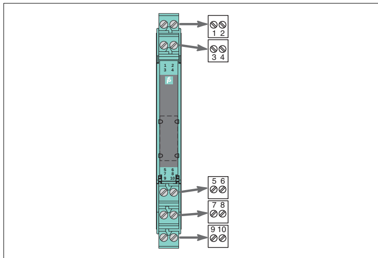
Figure 2.8 KC device housing (12.5 mm housing)
