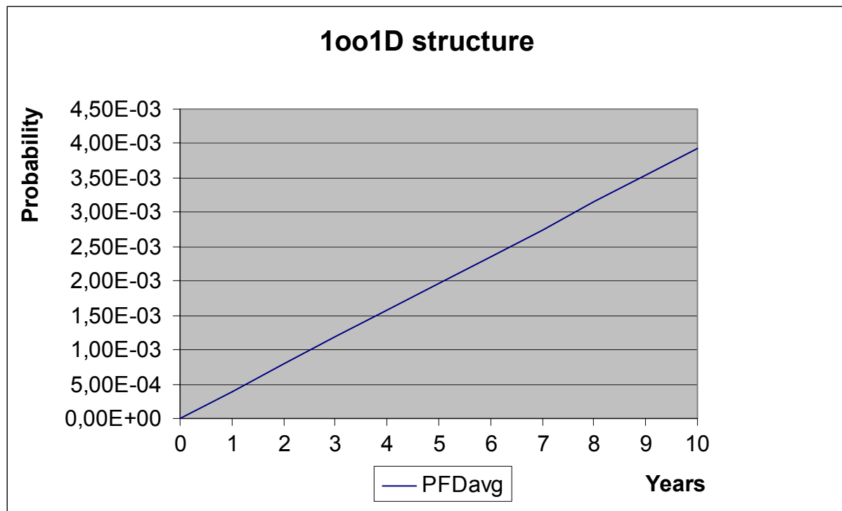
Figure 3: \text{PFD}_{\text{AVG}}(t)
