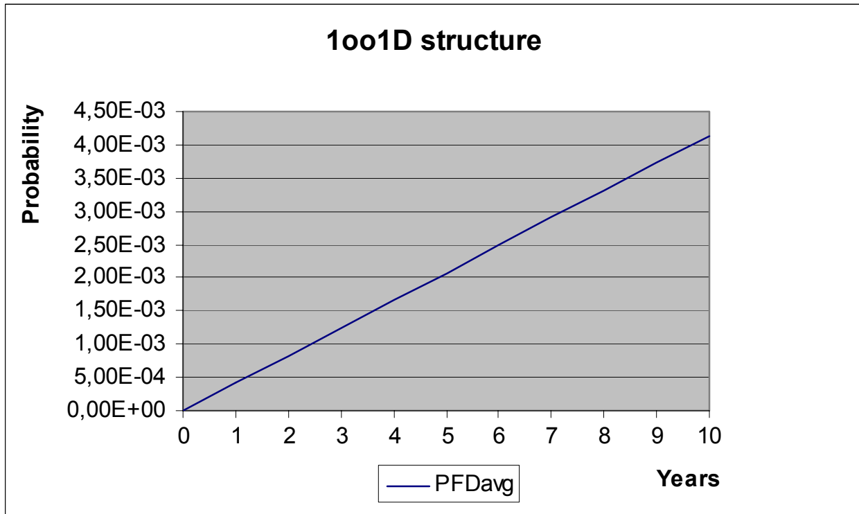
Figure 4: PFD_{AVG}(t)
