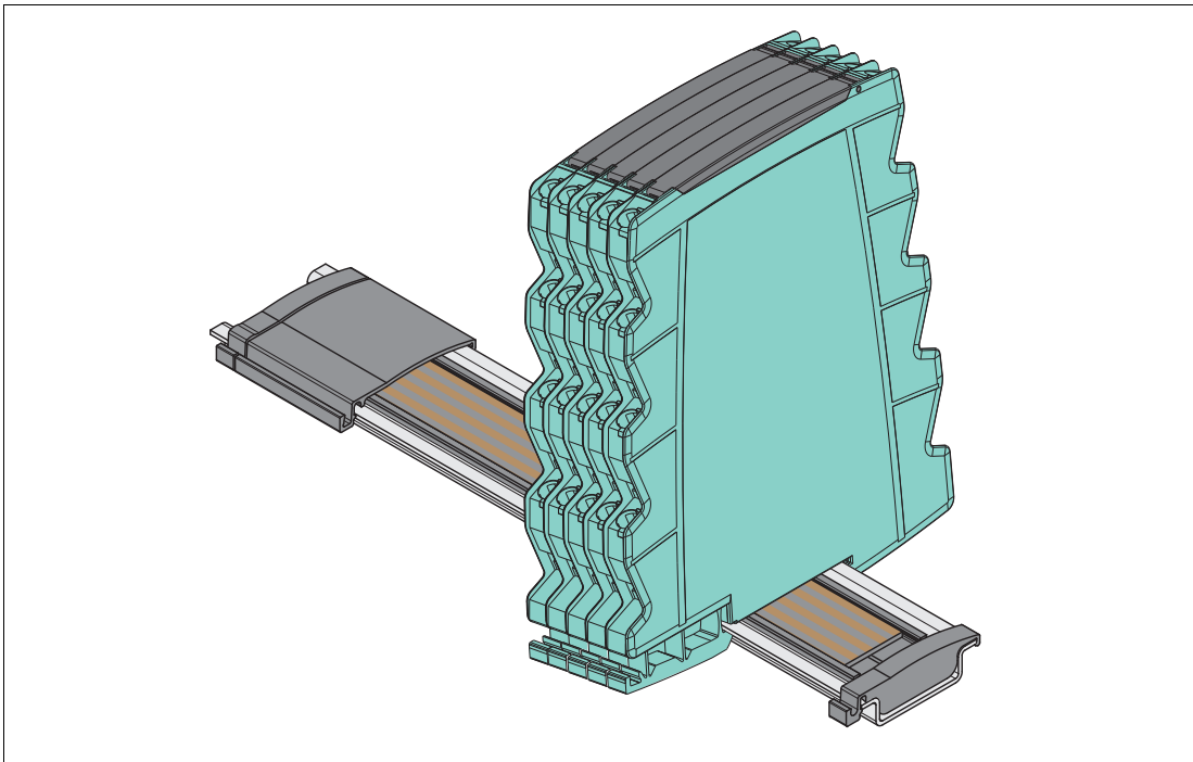
Figure 2.2 SC-System on DIN mounting rail with Power Bus
