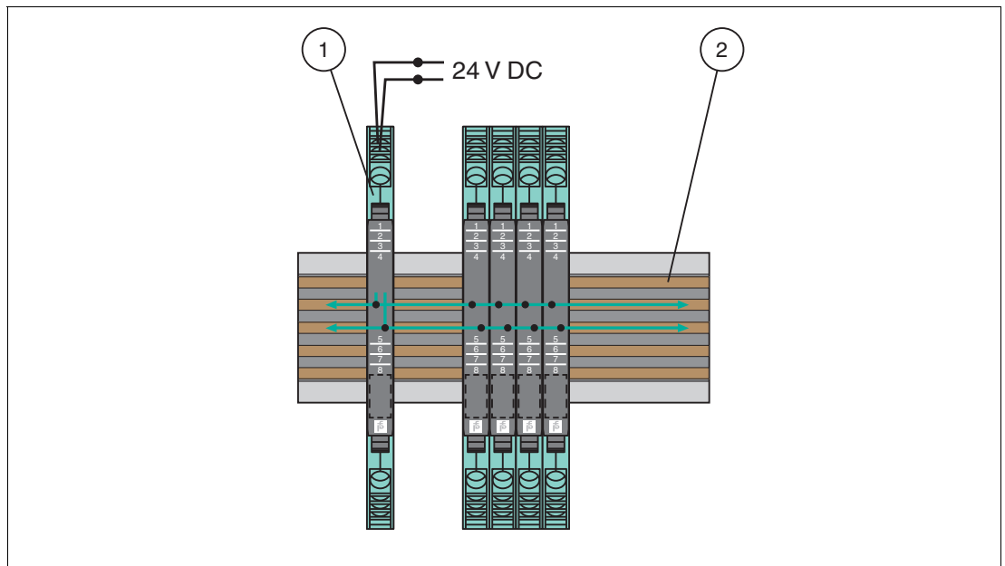
Figure 3.6 Non-redundant supply with isolator
