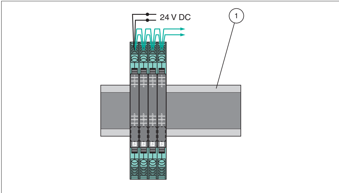
Figure 3.5 Conventional installation
