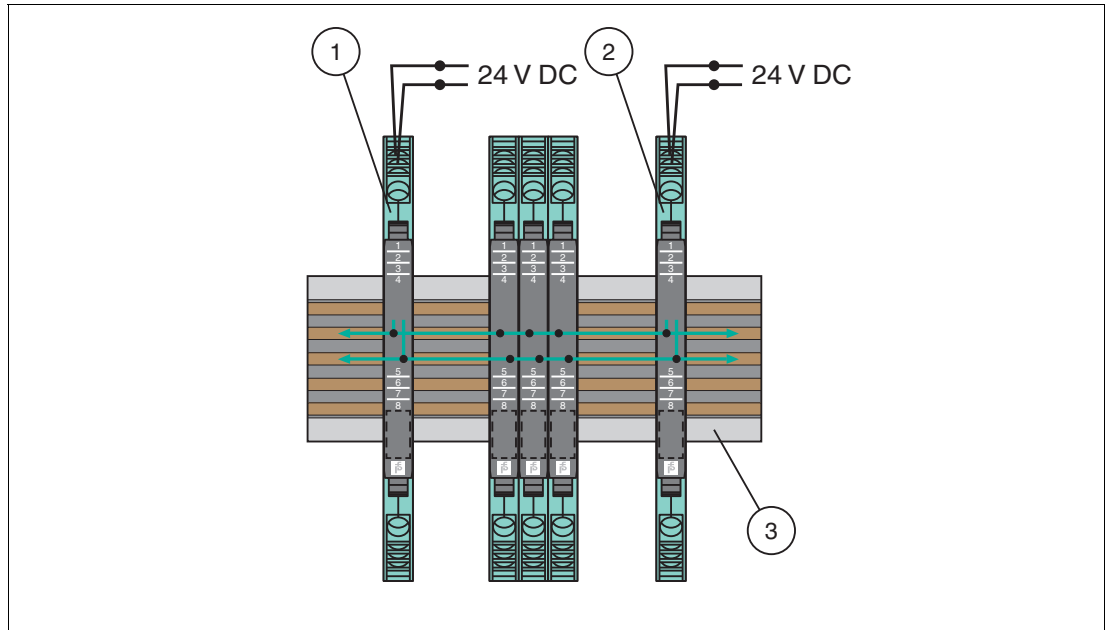
Figure 3.8 Redundant supply with power feed modules
