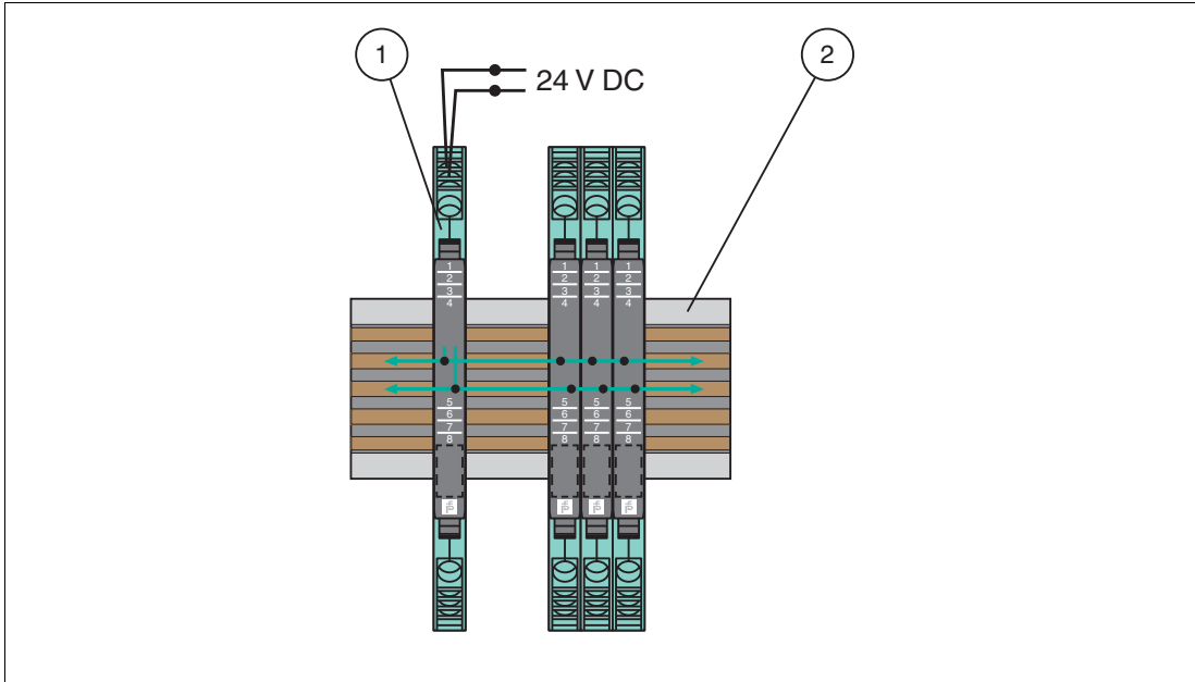
Figure 3.7 Non-redundant supply with power feed module
