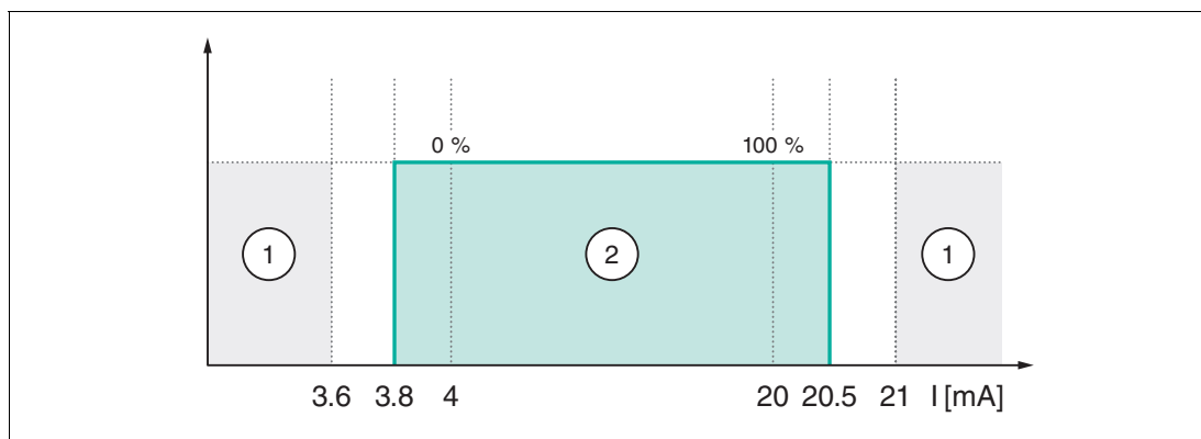
Figure 4.1 Signal ranges according to NAMUR NE43 (e. g. current signal)
