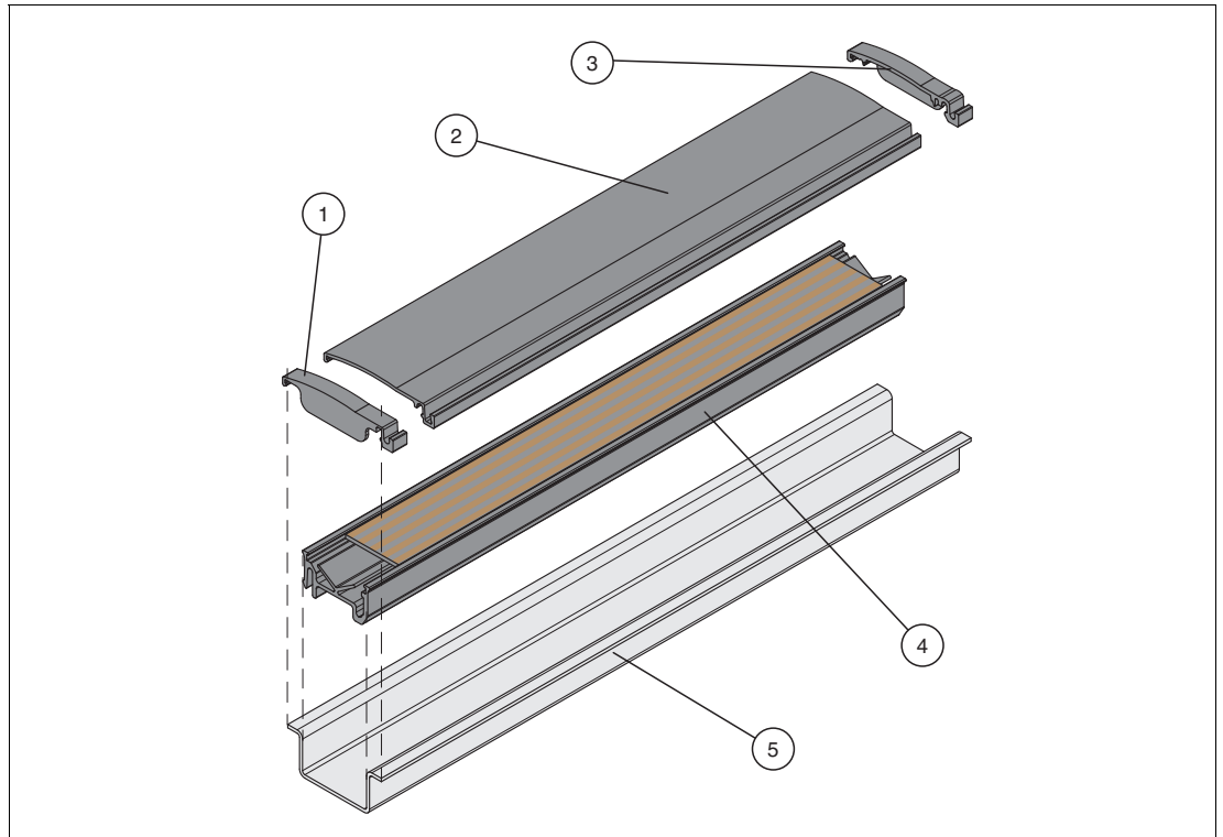
Figure 3.2 Example: Power Bus POWERBUS-SETH5.250
