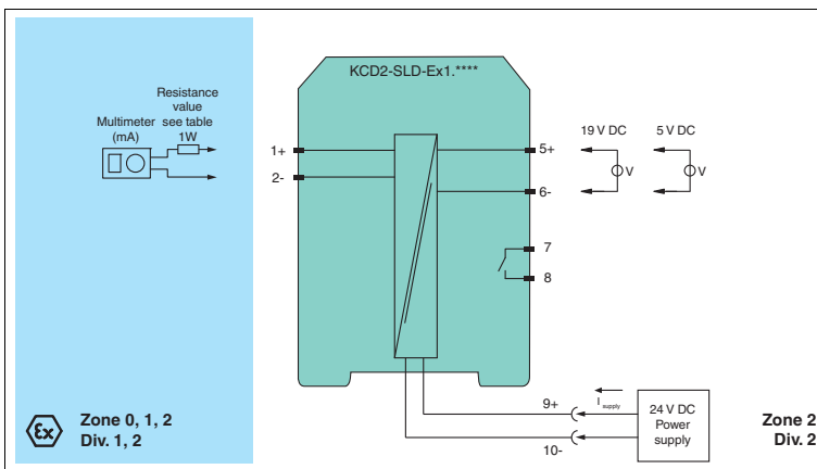
Figure 5.1 Proof test set-up for KCD2-SLD-Ex1.****
