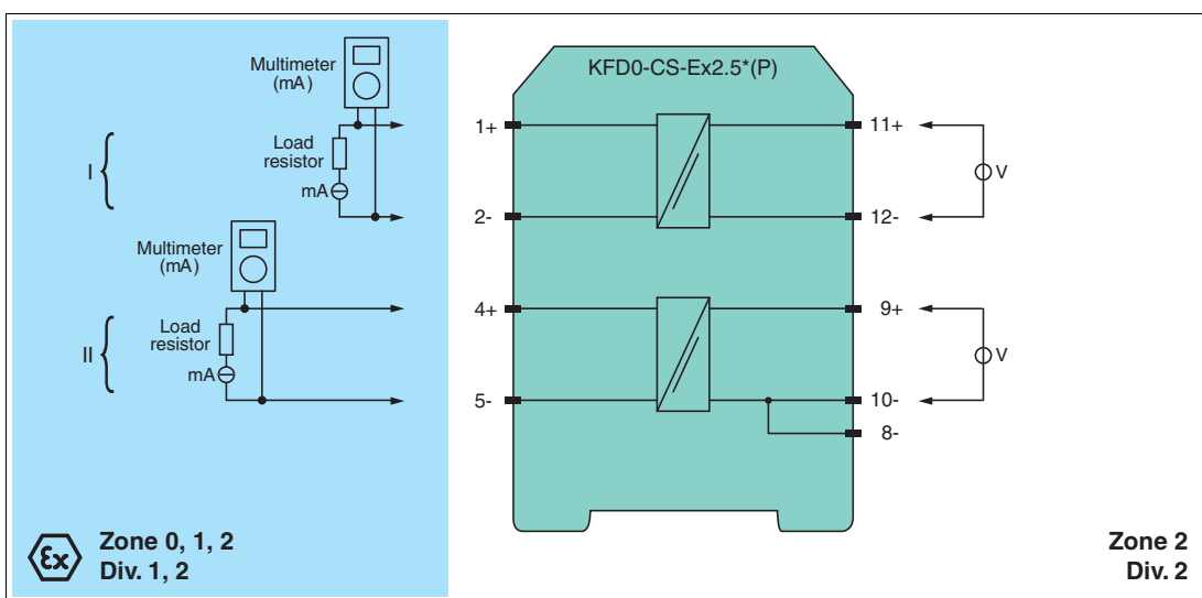
Figure 5.2 Proof test set-up for KFD0-CS-(Ex)*.5*(P)
