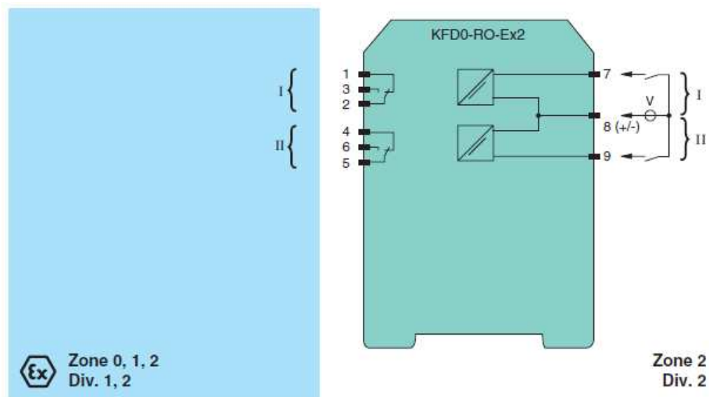
Fig. 1: Connection of the KFD0-RO-(Ex)2
