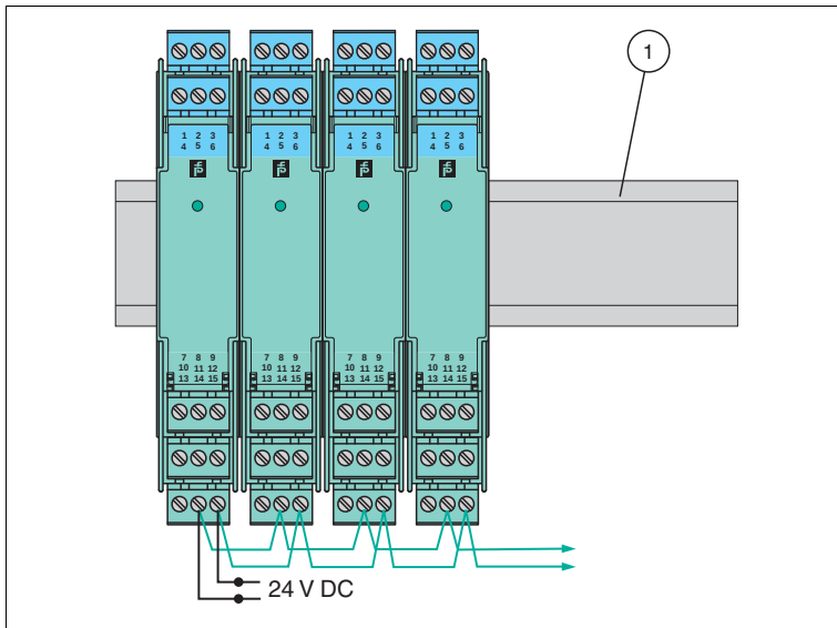
Figure 3.5 Conventional installation
