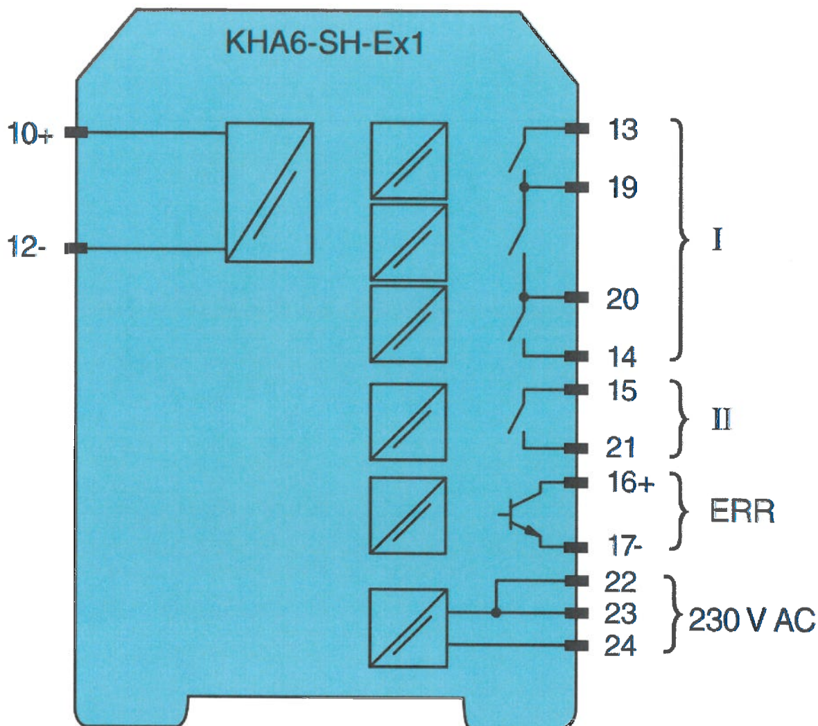
Figure 4: Block diagram of the unit KHA6-SH-Ex1 3
