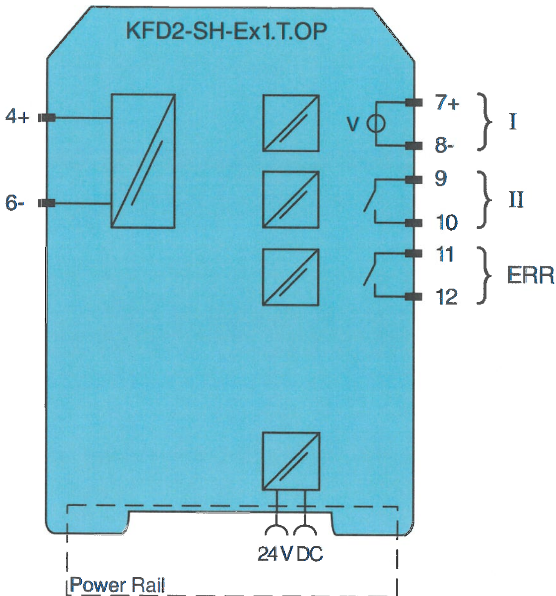
Figure 2: Block diagram of the unit KFD2-SH-Ex1.T.(OP) 1
