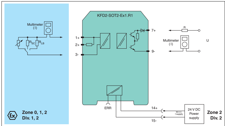
Figure 4.2 Proof test set-up for KFD2-SOT2-Ex1.R1
