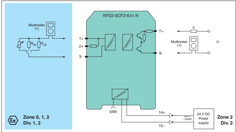
Figure 4.1 Proof test set-up for KFD2-SOT2-Ex1.N
