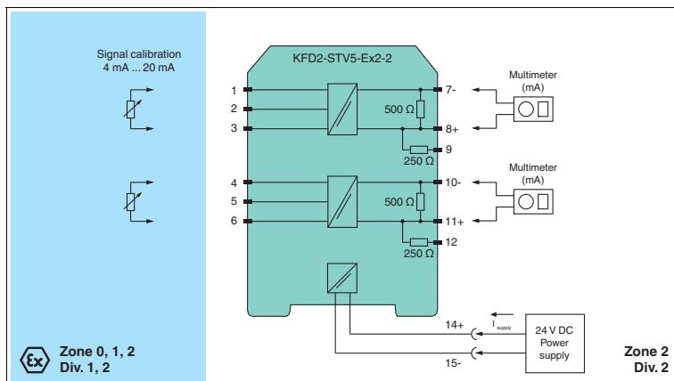
Figure 5.2 Proof test set-up for KFD2-STV5-(Ex)*-1 and KFD2-STV5-(Ex)*-2
