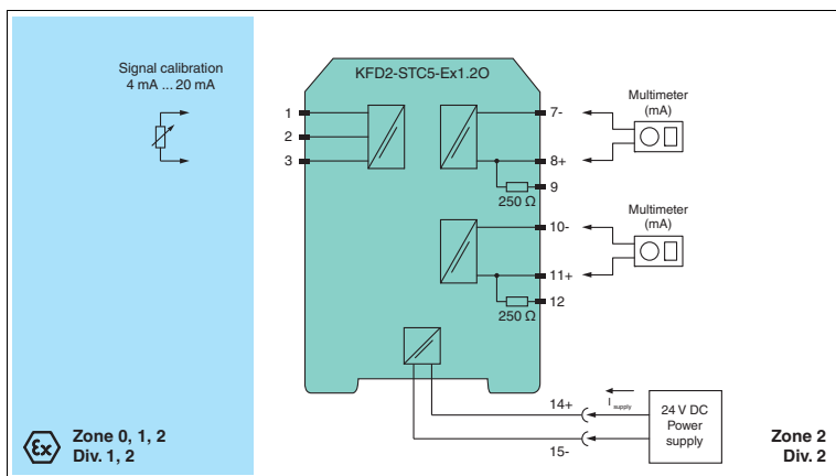
Figure 5.3 Proof test set-up for KFD2-STC5-(Ex) 1.20(.H)
