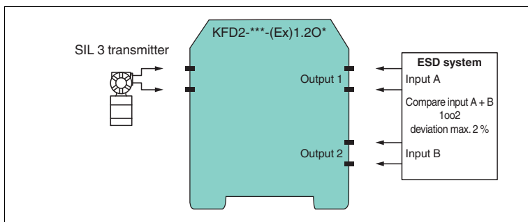
Figure 3.2 SIL 3 application
