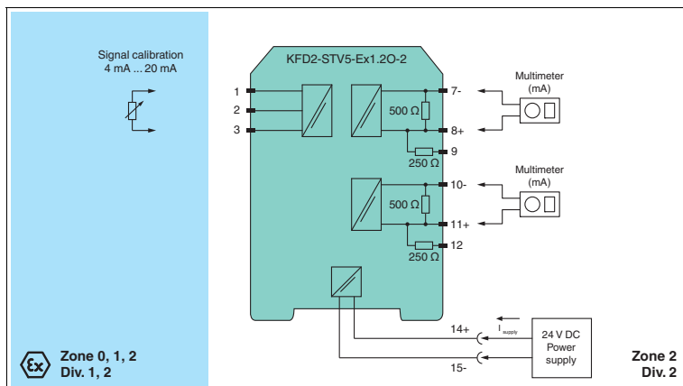
Figure 5.4 Proof test set-up for KFD2-STV5-Ex1.2O-1 and KFD2-STV5-Ex1.2O-2
