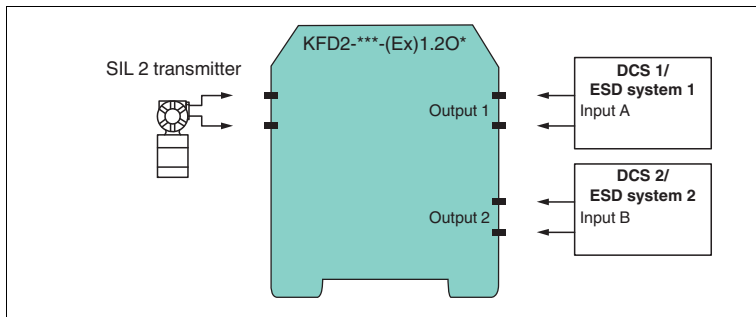
Figure 3.1 SIL 2 application
