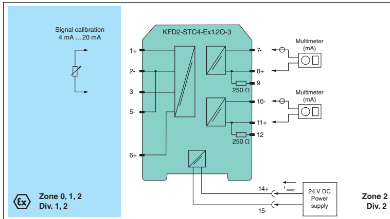
Figure 4.5 Proof test set-up for KFD2-STC4-(Ex)1.2O-3 and KFD2-STC4-(Ex)1.2O-Y*
