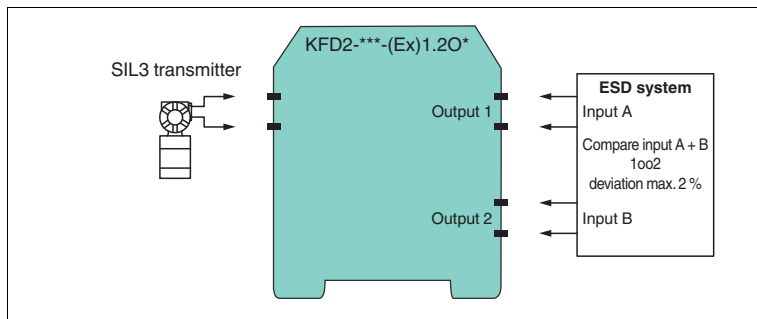
Figure 2.2 SIL3 application for KFD2-***-(Ex)1.2O* devices
