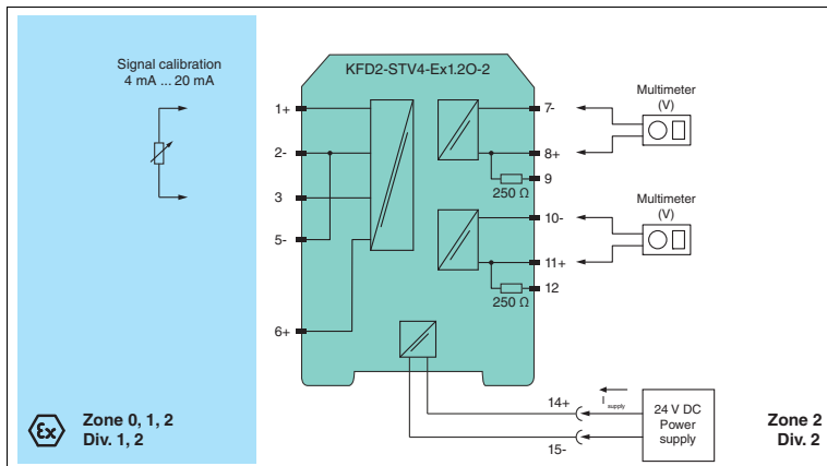
Figure 4.6 Proof test set-up for KFD2-STV4-(Ex)1.2O-1 and KFD2-STV4-(Ex)1.2O-2
