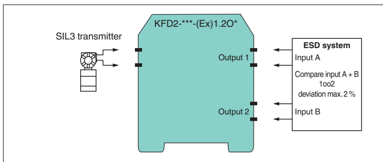
Figure 2.2 SIL3 application for KFD2-***-(Ex)1.2O* devices
