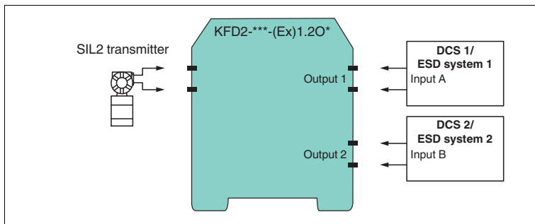
Figure 2.1 SIL2 application for KFD2-***-(Ex)1.2O* devices
