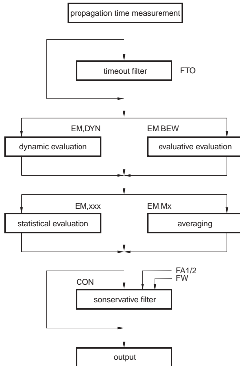
Figure 3.1: Evaluation methods
