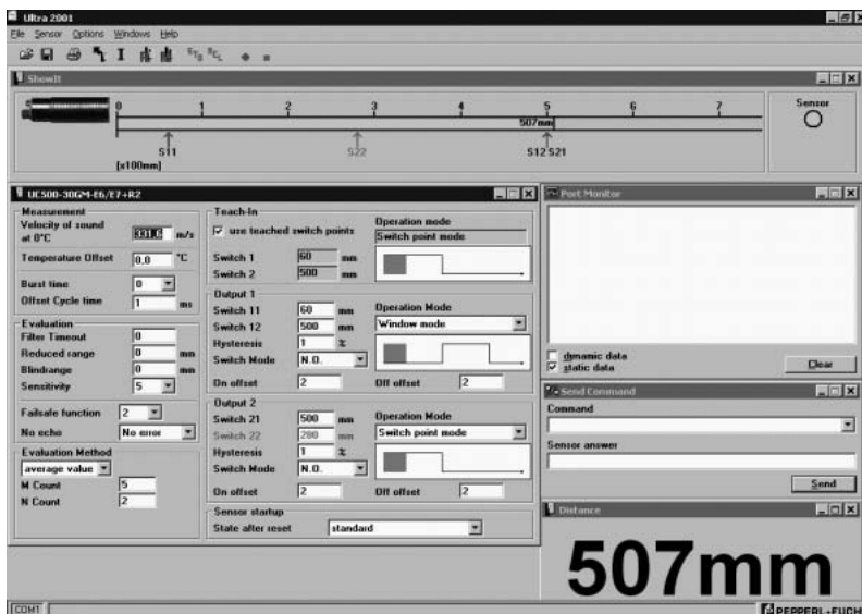
Figure 3.1: Screenshot with all activated windows
