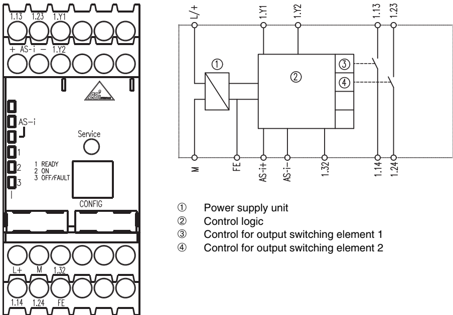
Figure 5.1: Terminal arrangement / block diagram of AS-interface safety monitor type 1 and type 3
