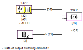
Figure 4.4: Logic device example
