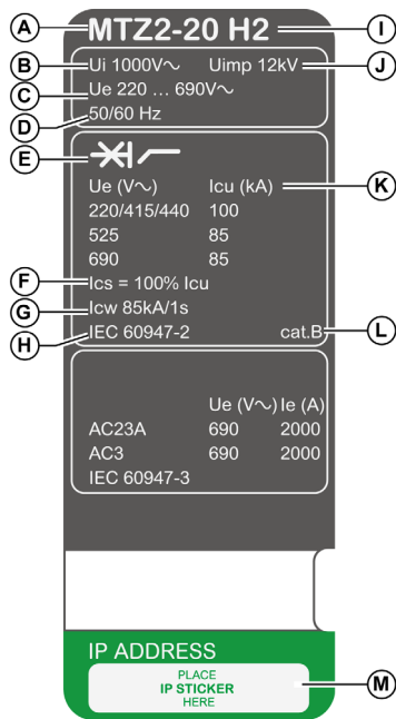
Circuit breaker rating plate
