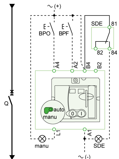
With manual reset
