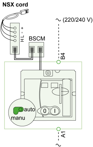
With communicating motor mechanism (MTc)
