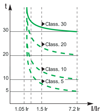
Standard trip time values
