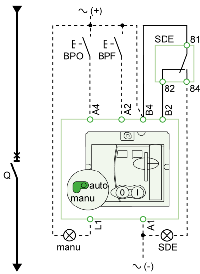
With automatic reset
