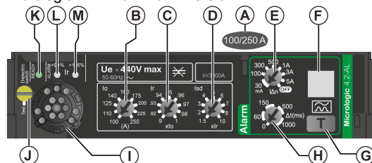
Micrologic 4.2AL 3P Alarm version
