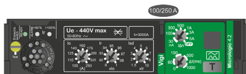
Micrologic 4 trip
