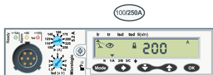
Micrologic 5 and 6
