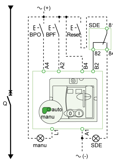
With remote reset
